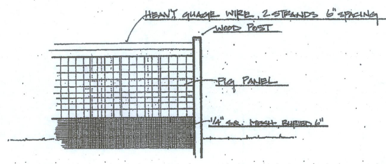
VEGETABLE GARDEN FENCE DETAIL (NTS)
